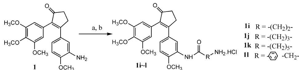
Scheme 2. Reagents and conditions: (a) HOOC-R-NHBoc, DCC, HOBT-H 2 O, DMF (b) 4 N HCl-dioxane, rt, 3 h.
