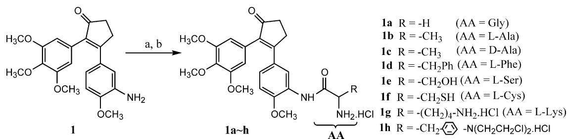
Scheme 1. Reagents and conditions: (a) protected amino acid (N-Boc-gly for 1a , N-Boc-L-Ala for 1b , N-Boc-D-Ala for 1c , N-Boc-L-Phe for 1d , N-Fmoc-O-tert-Bu-L-Ser for 1e , N-Boc-S-trityl-L-Cys for 1f , diBoc-L-Lys for 1g , and N-Boc-Melphalan for 1h ), DCC, HOBT-H 2 O, DMF; (b) 4 N HCl-dioxane, rt, 3 h (for 1a–d and 1g–h ); piperidine/CH 2 Cl 2 then 4 N HCl-dioxane, rfx, 3 h (for 1e ); or 3 N HCl-aq. AcOH, 90 °C, 1.5 h (for 1f ).
