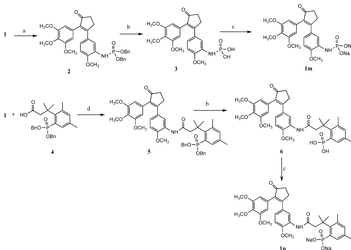
Scheme 3. Reagents and conditions: (a) P 2 O 7 Bn 4 , TEA, MeCN, rfx; (b) TMS-Cl, NaI, acetonitrile, rt; (c) THF, MeONa, rt; (d) 3-[2'-(dibenzylphosphono)oxy-4',6'-dimethylphenyl]-3,3-dimethylpropionic acid ( 4 ), 15 DCC, HOBt-H 2 O, CH 2 Cl 2 .
