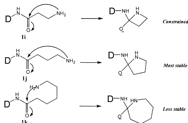
Figure 2. Possible pathways for generation of 1 from prodrugs 1i–k ( D , a parent drug).
