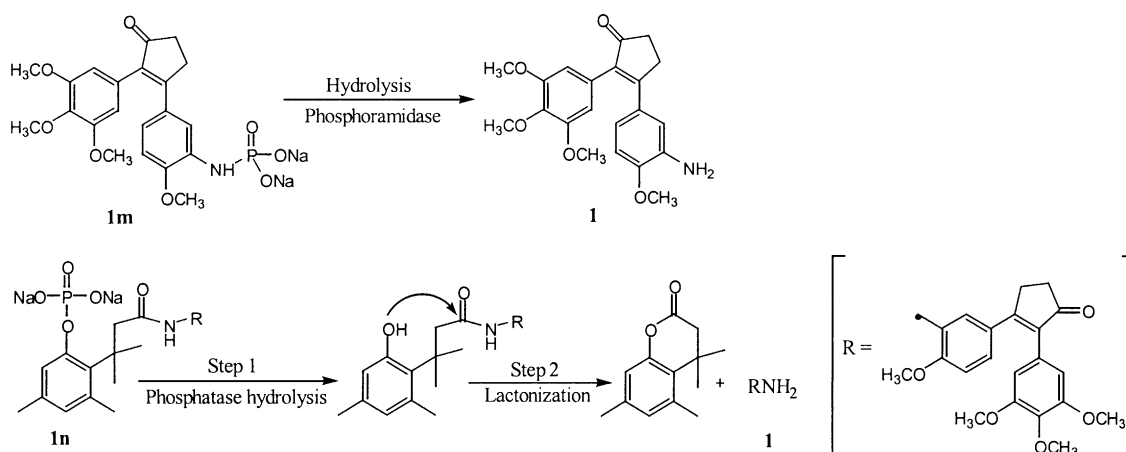
Figure 3. Possible pathways for generation of 1 from prodrugs 1l and 1m .
